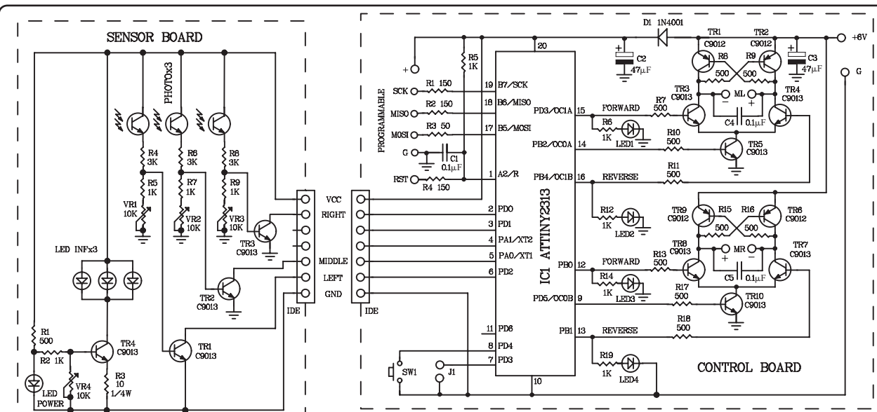
Figure 1. AVR1 Super Sumo Robot Circuit
