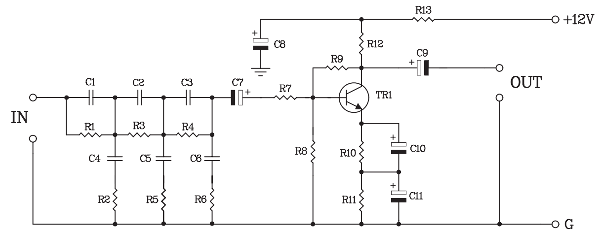
Figure 2. The loudness (stereo) circuit
