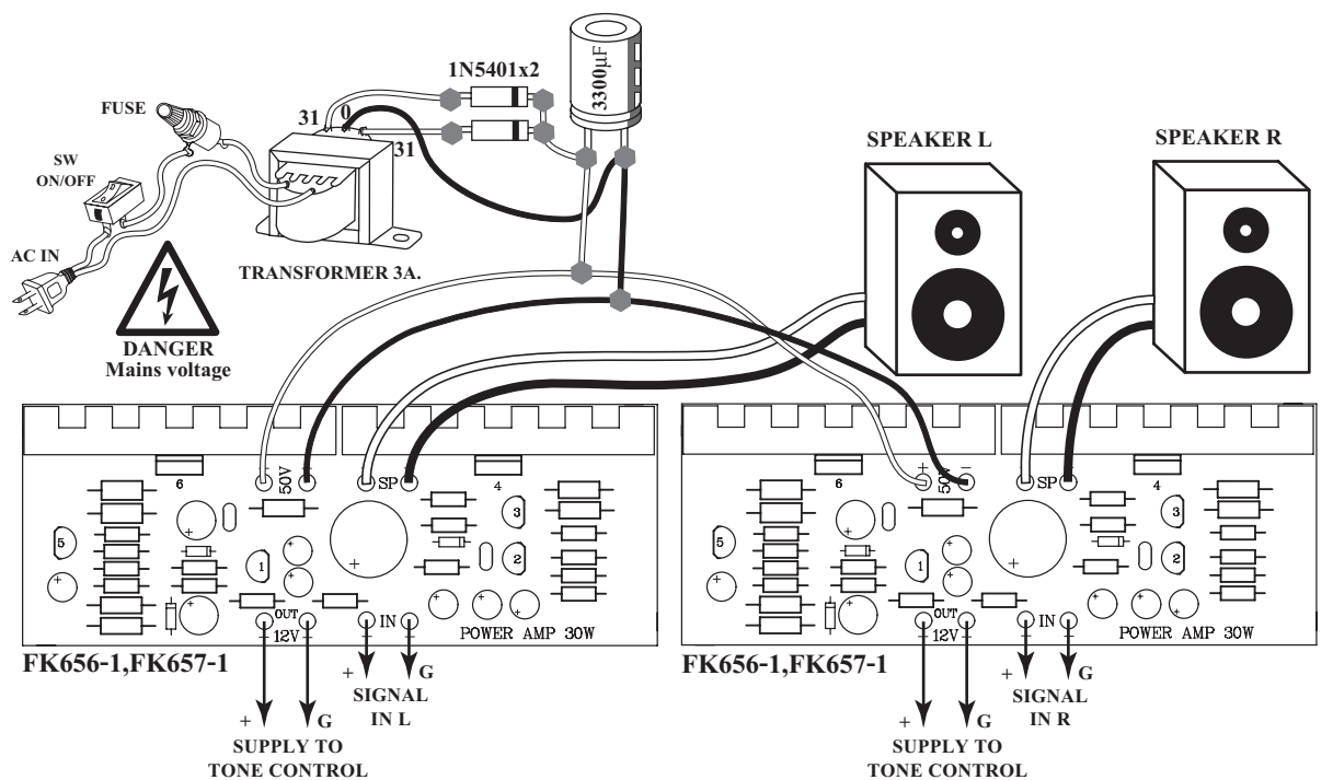
Figure 3. Connections
