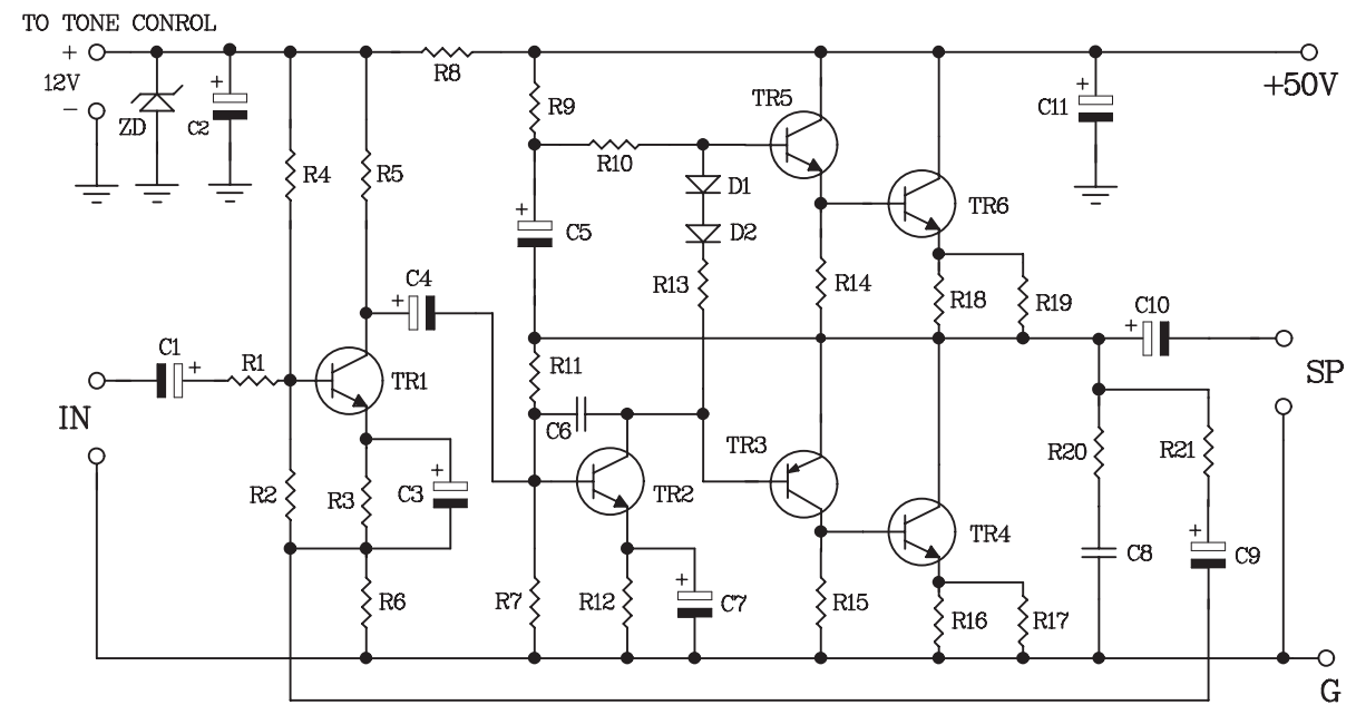
Figure 2. The power amp OTL 30W R1% circuit
