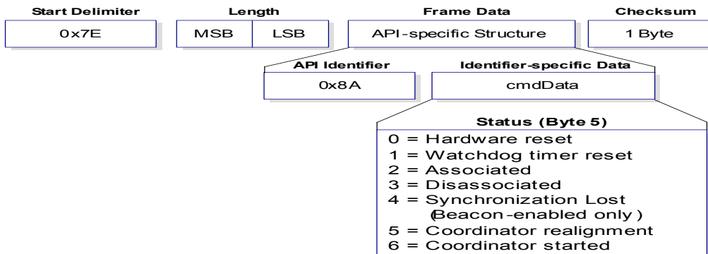
Figure 3-04. Modem Status Frames
