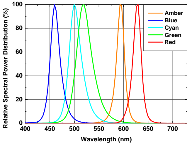
Wavelength Characteristics
