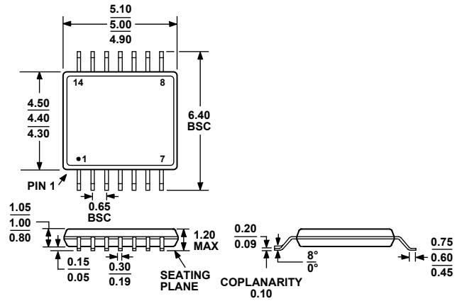
Figure 70. 14-Lead Thin Shrink Small Outline Package [TSSOP] (RU-14)
