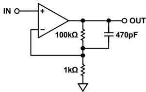
Figure 52. Test Circuit: First-Order Low-Pass Filter, \times 101 Gain and 3 kHz Corner Frequency
